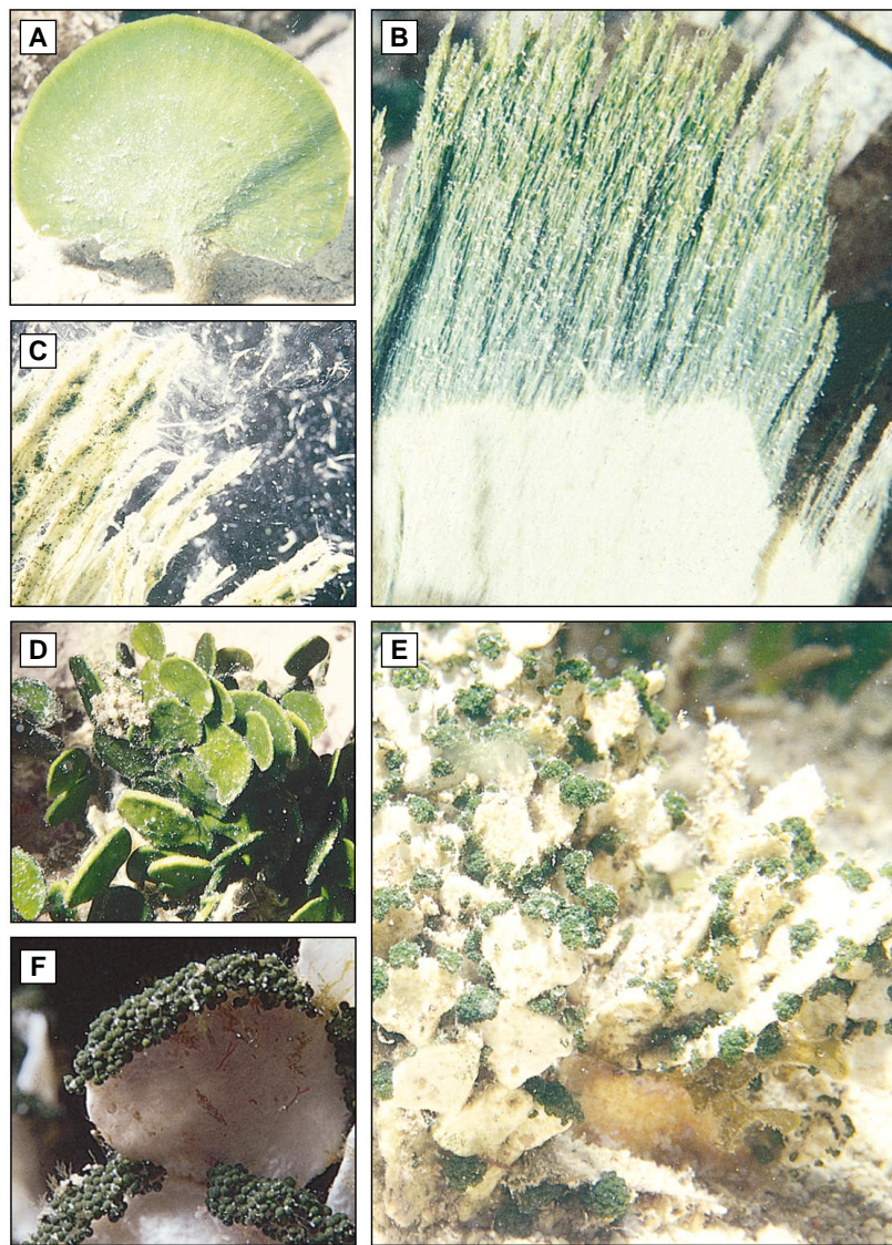
Fig. 2. Photographs of green algae before and during gamete release. (A) through (C) Udotea caribaeae . (A) A typical green thallus of nonfertile plant. (B) A close-up of green gametangia of fertile female is shown. This condition developed overnight as the entire protoplasmic contents migrated from the thallus below (now white). (C) An extreme close-up of gamete release shows individual gametes (green spots) visible within mucilaginous streams. (D) through (F) Halimeda . (D) Nonfertile Halimeda tuna . (E) Fertile H. simulans , with clustered gametangia along blade margins; (F) A close-up of gametangial release for U. caribaeae highlights the earlier spawning of males (27).
